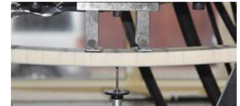
Infused panels undergoing flex testing at the renowned Wolfson Unit MTIA in Southampton – these test panels are just 75mm wide and 600mm long but can withstand a load of 300kgs
