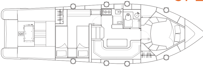
Lower deck
